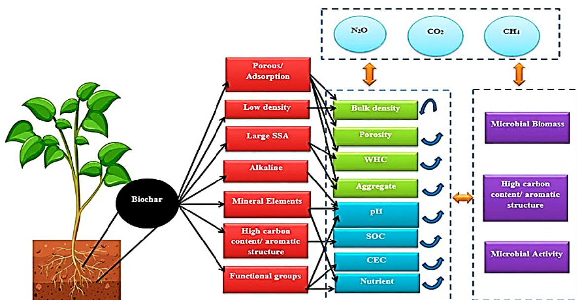
Figure 4. The impact of biochar addition on the physicochemical and biological properties of soil; Carbon dioxide ( \text{CO}_2 ), cation exchange capacity (CEC), nitrous oxide ( \text{N}_2\text{O} ), methane ( \text{CH}_4 ), soil organic carbon (SOC), specific surface area (SSA), water-holding capacity (WHC) [25]
